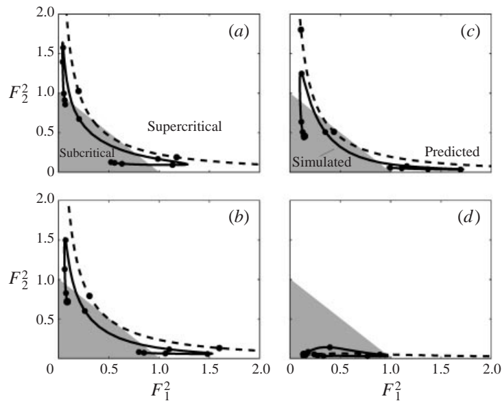
FIGURE 14. Simulated (solid) and predicted (dashed) solution curves plotted on a Froude number plane for (a) q_r = 0.59 , (b) q_r = 1.02 , (c) q_r = 1.92 and (d) q_r = 1.73 . In the shaded region of the Froude number plane the flow is subcritical. Dots along the curves mark approximately 6 m intervals along the channel. Plots (a–c) are maximal exchange solutions and plot (d) is a submaximal exchange solution.
