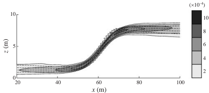
FIGURE 8. Contours of K_m = K_T (in \text{m s}^{-1} ) for q_r = 1.92 , overlain with isopycnals between 0.1 and 0.4 \text{ kg m}^{-3} . Note the symmetry of the distribution of K_m about the contraction, and the close correspondence in the positions of maximum K_m and the pycnocline.
